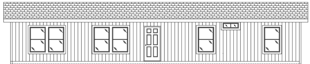
FRONT SIDEWALL
